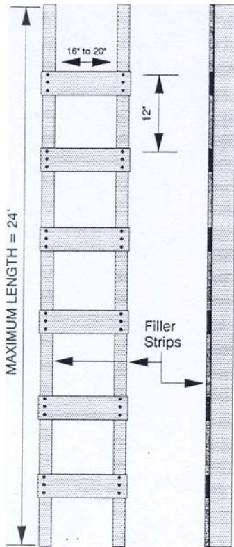
SINGLE CLEAT LADDER
