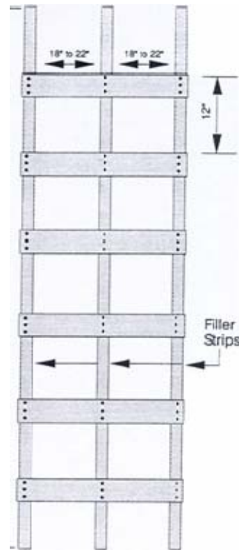
DOUBLE CLEAT LADDER
